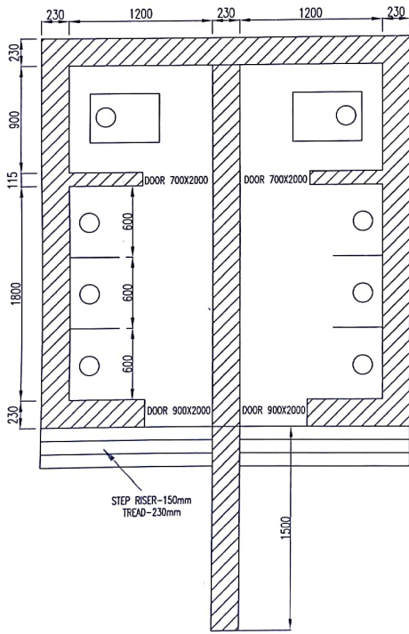
PLAN
