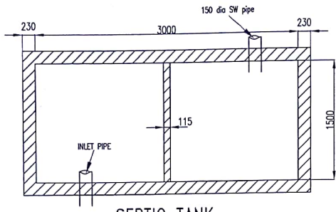
SEPTIC TANK
