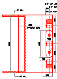
ABUTMENT CAP PLAN A1 & A2
