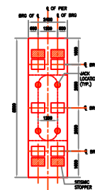
TYPICAL PIER CAP PLAN P1 TO P7 & P11 TO P17
