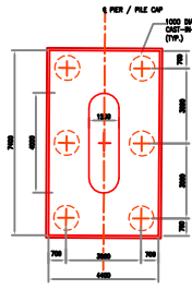
TYPICAL PLAN OF PILE GROUP (AT VIADUCT SPAN)
